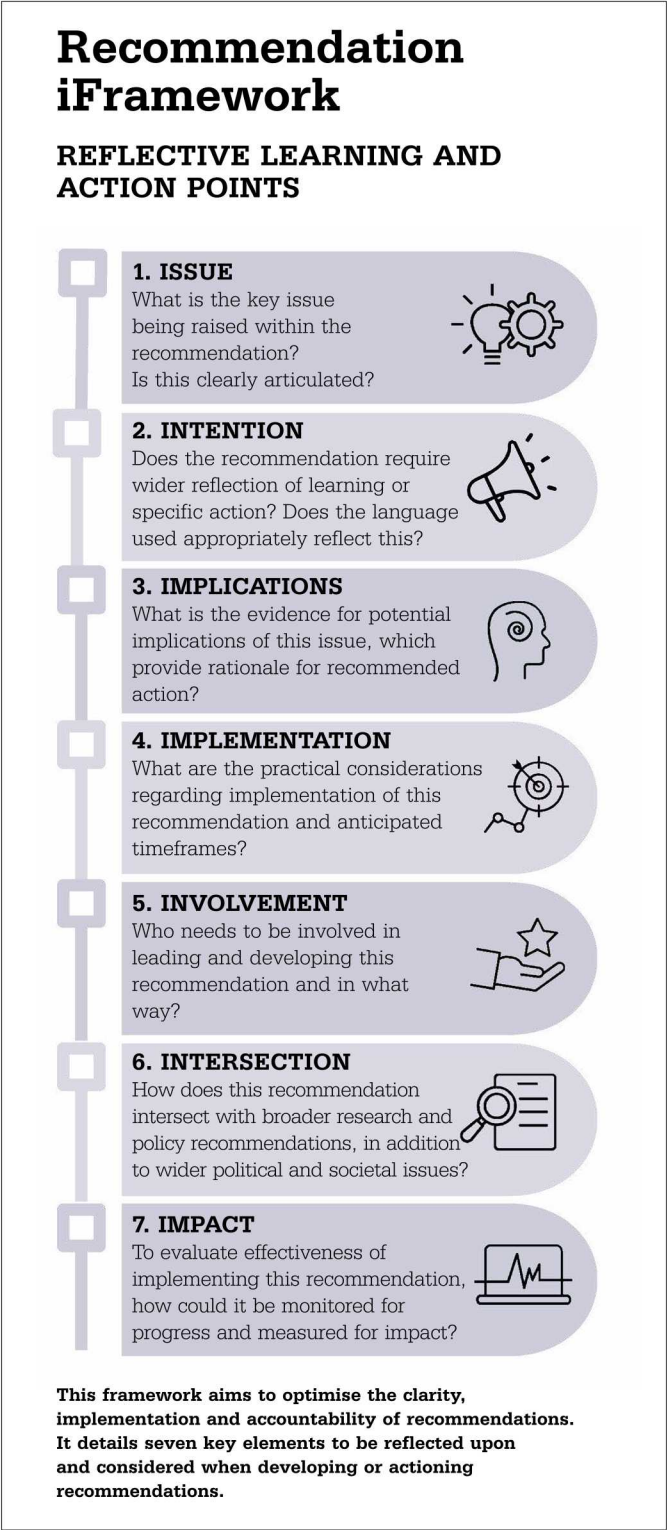
Figure 1. Recommendation iFramework
